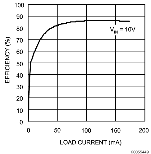
Efficiency vs Load ( V_{OUT} = 15V ) - "Y"
