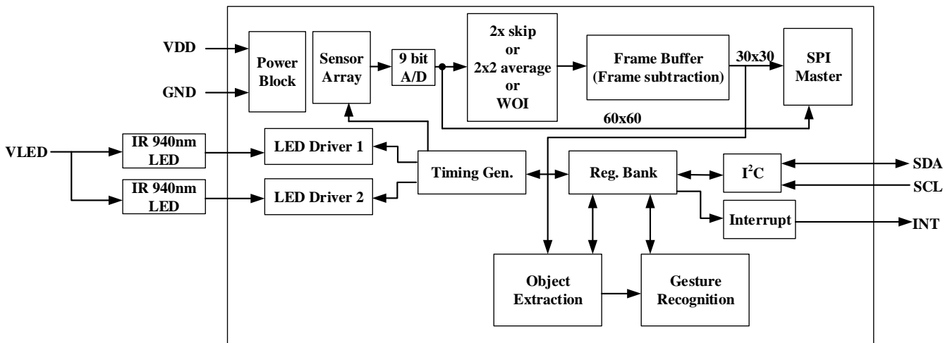
Figure 1. Architecture Block Diagram
