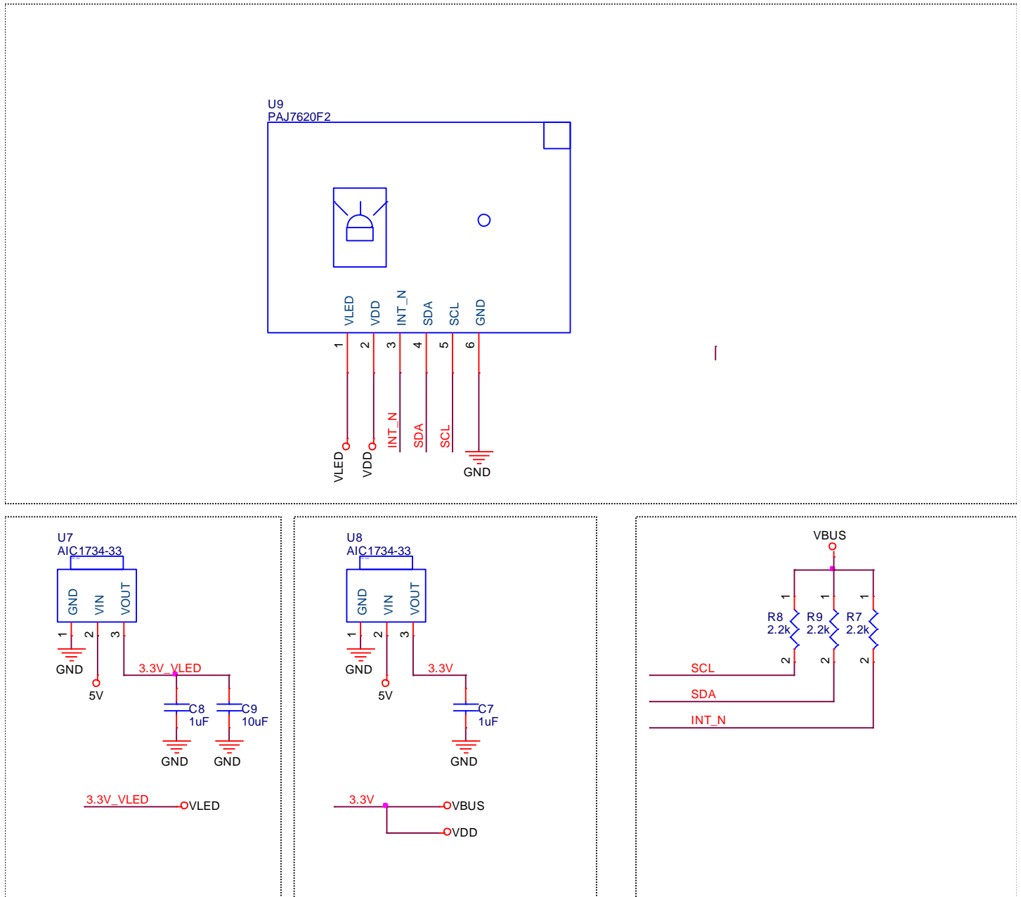
Figure 7. PAJ7620F2 Application Circuit
