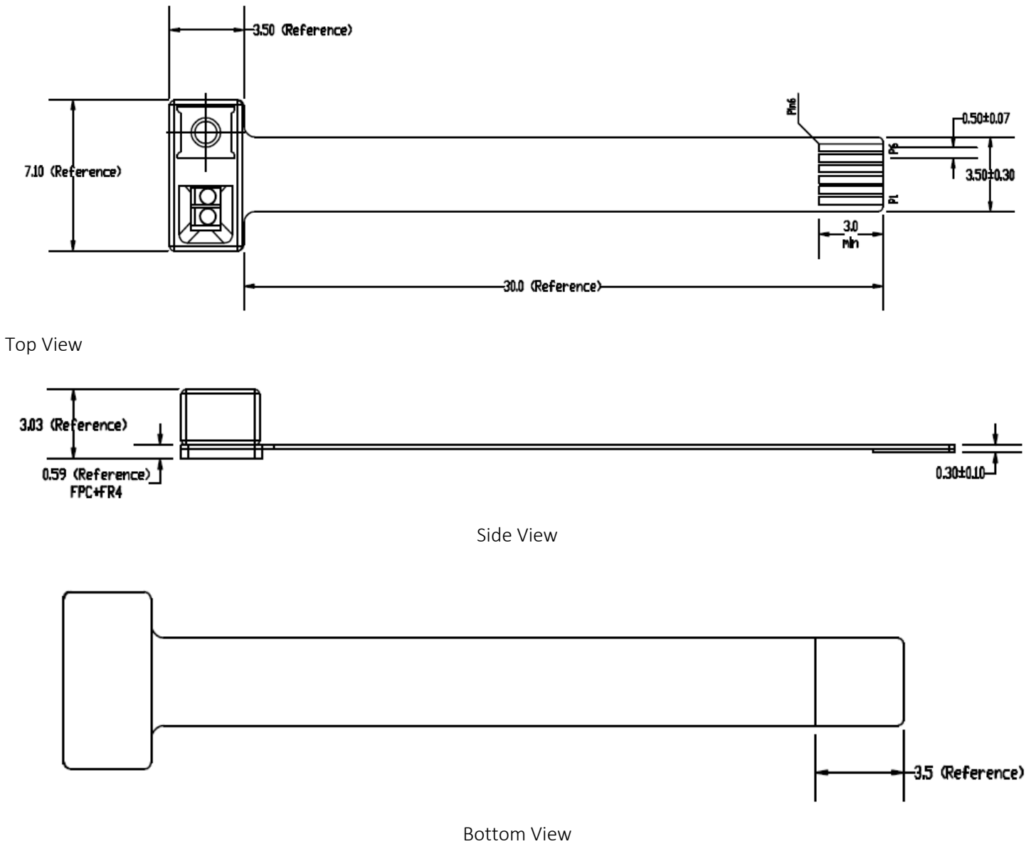
Figure 3. PAJ7620F2 Package Outline Diagram
