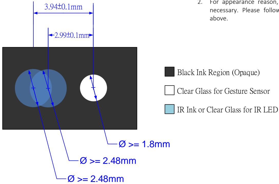
Figure 5. PAJ7620F2 Mechanical Design Guide (IR Ink Suggestion)
