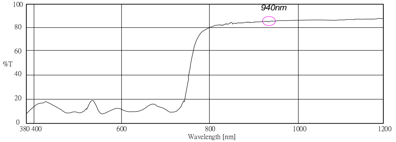
Figure 6. IR Ink Spectrum
