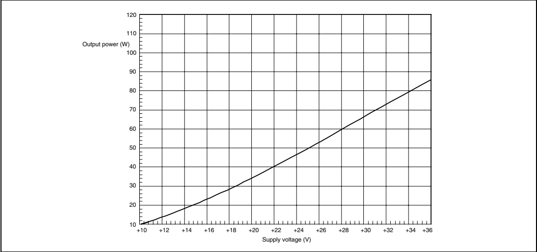
Figure 12. Output power (THD = 10%) vs. supply voltage
