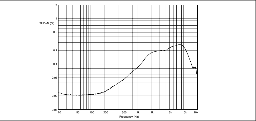
Figure 14. THD vs. frequency (1 W)
