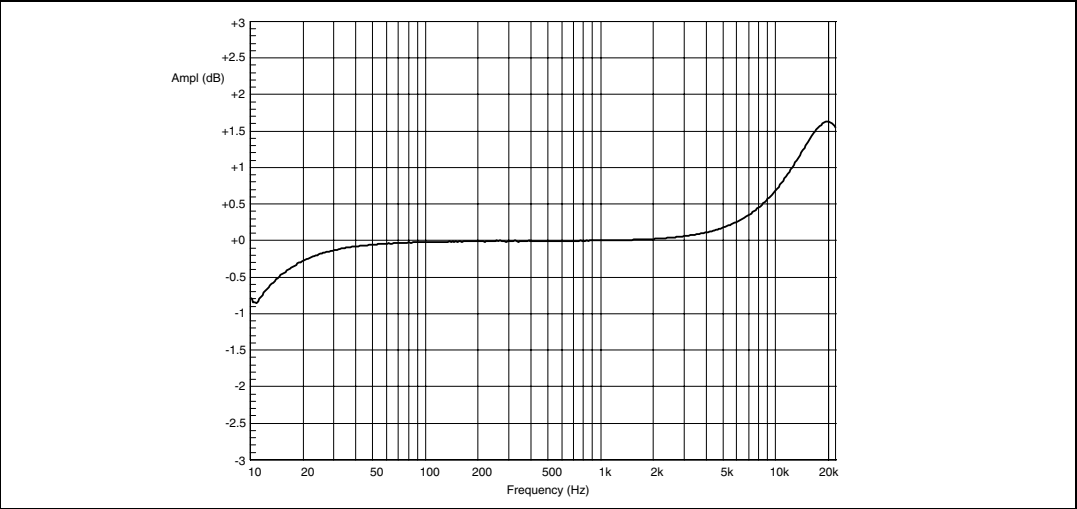
Figure 16. Frequency response
