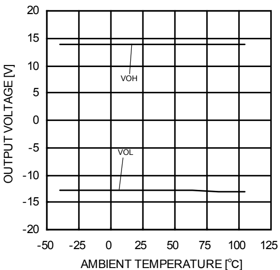
Figure 74. Maximum Output Voltage - Ambient Temperature (VCC/VEE=+15V/-15V, RL=2kΩ)
